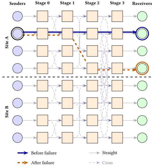
Figure 2: A butterfly topology [40] used for research on FABRIC—the largest-known single-experiment topology on the testbed. CRINKLE is used to easily verify the flow of traffic before and after a failure of a switch, and identify that the stage 2 switch is the failure.
