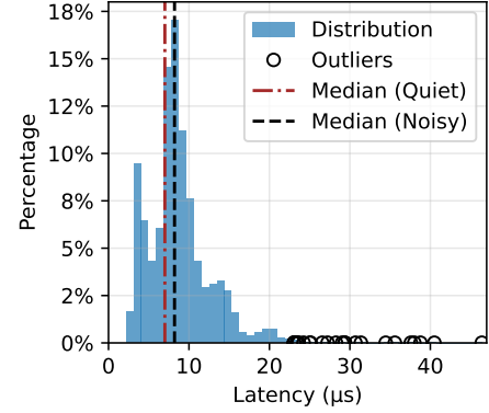
Figure 6: Latency distribution of sampled packets in a noisy environment, with a median of 8.21 \mu\text{s} . Shown is the median of 7 \mu\text{s} for the same setup in a quiet environment, which had a similar sub- 22 \mu\text{s} distribution but fewer outliers.
