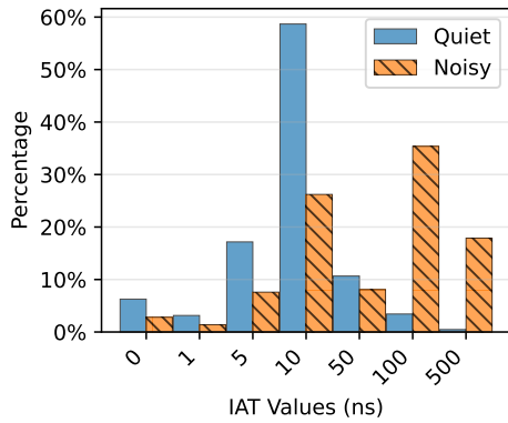
Figure 9: The run-to-run variation in packet IATs (inter-arrival times) at 40 Gbps when there is no other tenant traffic (“Quiet”) and when there is a varying 35–50 Gbps of other-tenant traffic on a 100 Gbps link (“Noisy”). Measured on FABRIC using hardware timestamping of a Mellanox ConnectX-6 SR-IOV virtual function, which was synchronized via PTP through the VM to a GPS time source [52].
