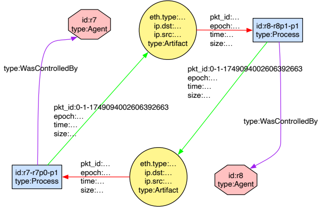
Figure 4: CRINKLE-produced provenance graph with most values elided to reduce clutter. Read from top-left to bottom-right, the graph indicates that r7 is forwarding packets from r8 back towards r8. This example is referenced and explained in Section 4.2.
