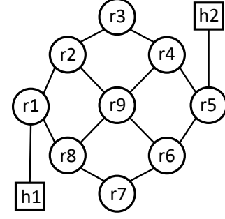
Figure 8: An abstract topology of two endpoints separated by multiple routers and paths, used for the case studies and user study. It balances complexity (6 paths across 9 routers) with size (11 nodes).
