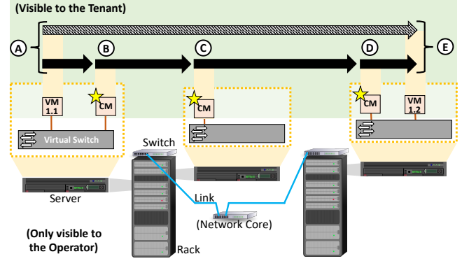
Figure 3: CRINKLE nodes decompose virtual links to obtain granular observations about packet propagation. The lower part of the figure shows infrastructure that is only visible to the testbed operator, but whose configuration and behavior affects the testbed’s users.
