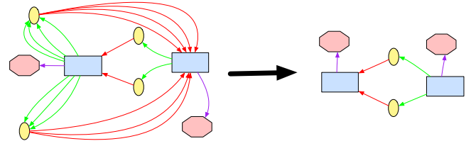
Figure 5: Demonstration of TCP flow abstraction. The filtering collapses multiple packet edges into a single flow-level edge.
