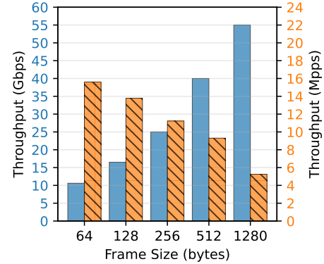
Figure 7: The throughput of the monitor at different frame sizes. The throughput is measured in Gigabits per second on the left y-axis, and in Millions-of-packets per second on the right y-axis.
