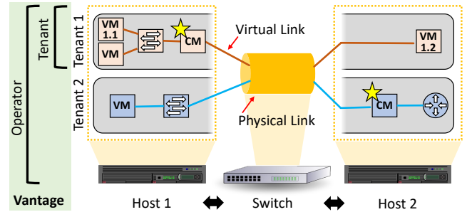
Figure 1: CRINKLE mitigates the restricted vantage that tenants have when debugging their network. CRINKLE works by controlling the behavior of opportunistic, ephemeral virtual resources for network debugging—here, VMs labeled as “CM” (for CRINKLE Monitor).
