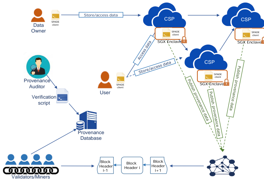
Figure 1: Prov-Trust Architecture.
