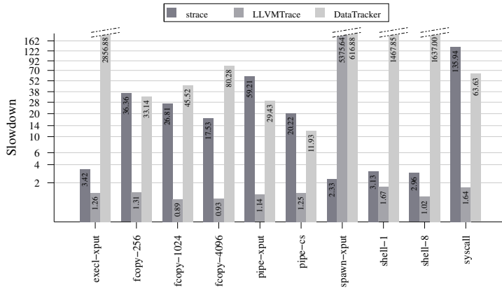
Fig. 2: Slowdown for the individual UnixBench tests.
