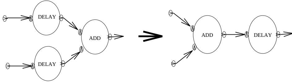
Figure 2.11: Example SIL transformation: retiming.
