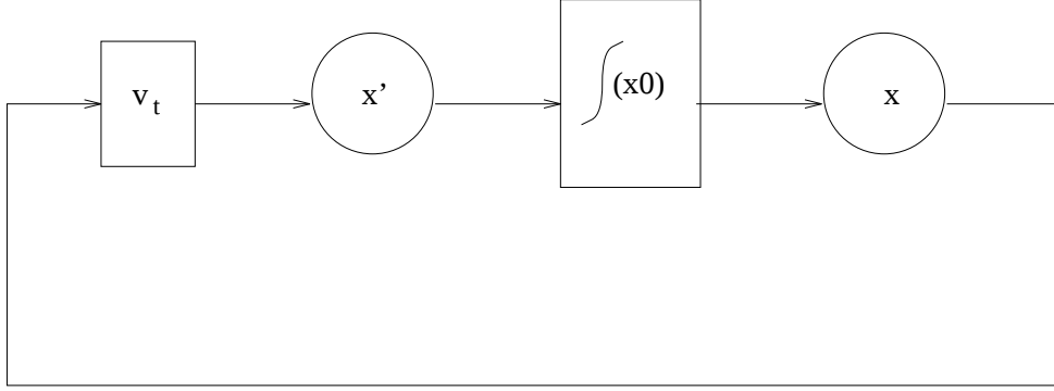
Figure 8.8: Constraint net for modeling integral computation over continuous time
