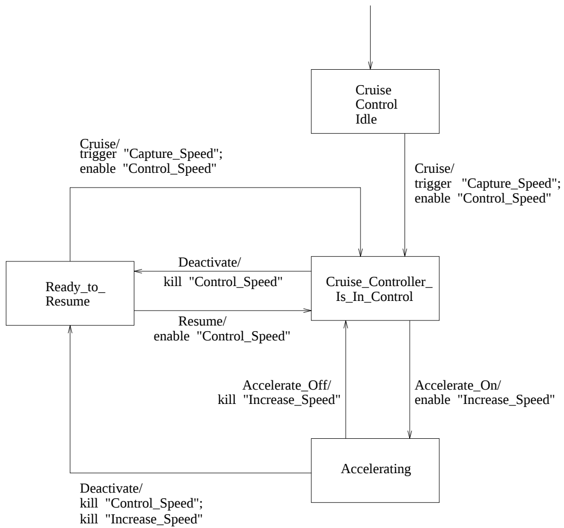
Figure 8.6: STD for cruise control of an automobile
