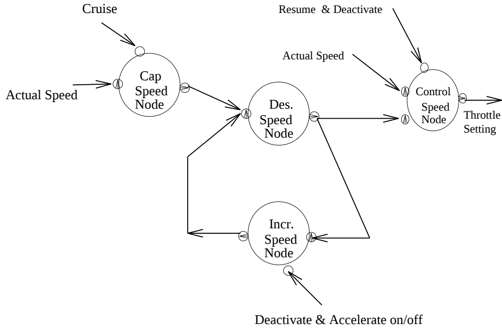
Figure 8.7: SIL for cruise control of an automobile
