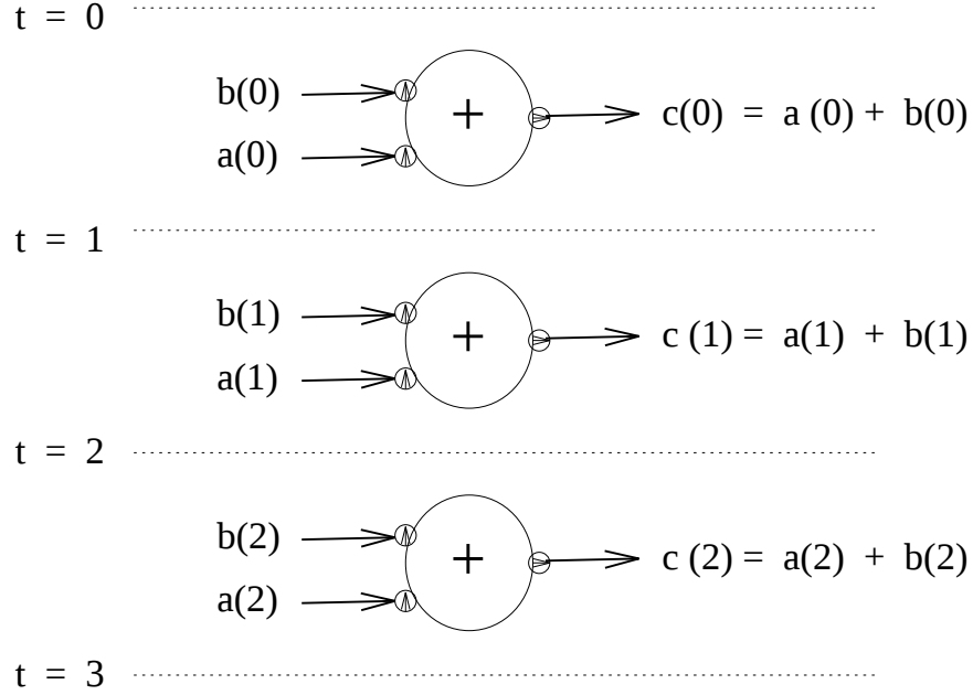
Figure 2.6: Combinational adder: SIL graph repeated over clock cycles.
