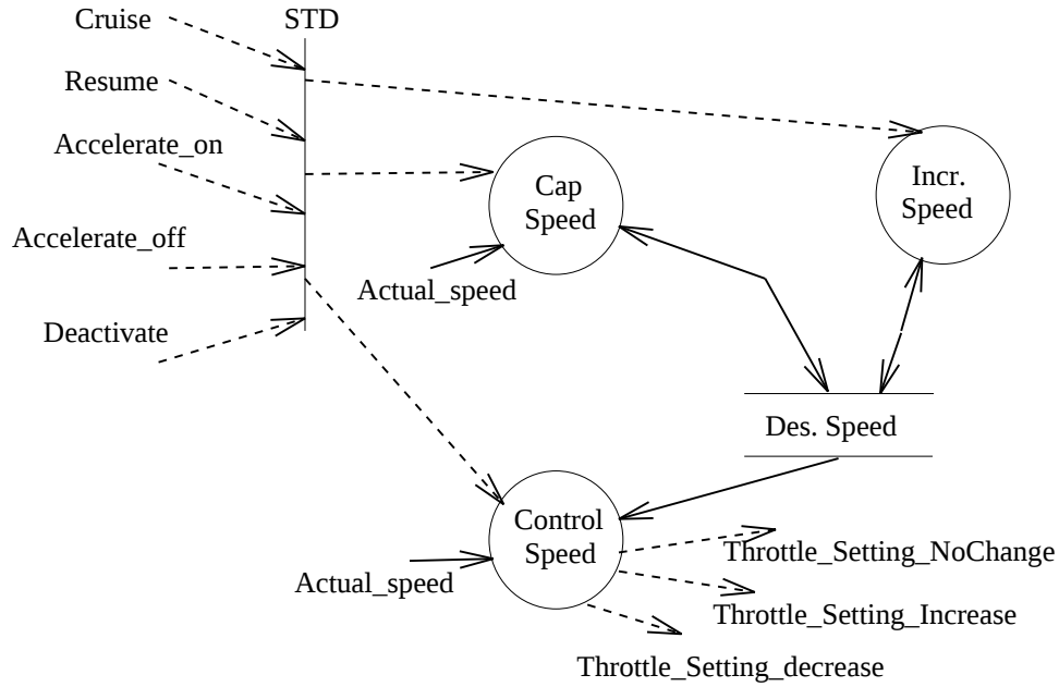
Figure 8.5: DFD for cruise control of an automobile
